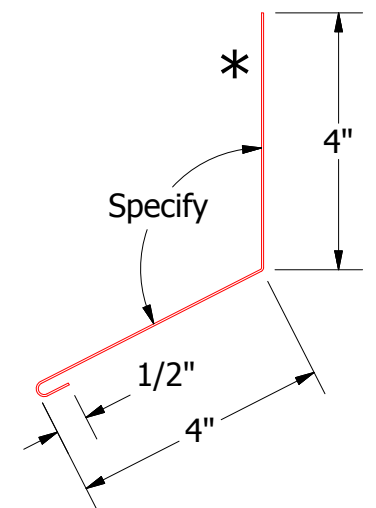
MDA500-Headwall Trim
