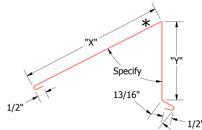
Shed Ridge Cap MDA342: 2:12-6:12 Slope "X"=7" , "Y"=4 1/8" MDA344: 6:12-9:12 Slope "X"=8" , "Y"=4 3/8" MDA346: 9:12-12:12 Slope "X"=9" , "Y"=4 1/2"
