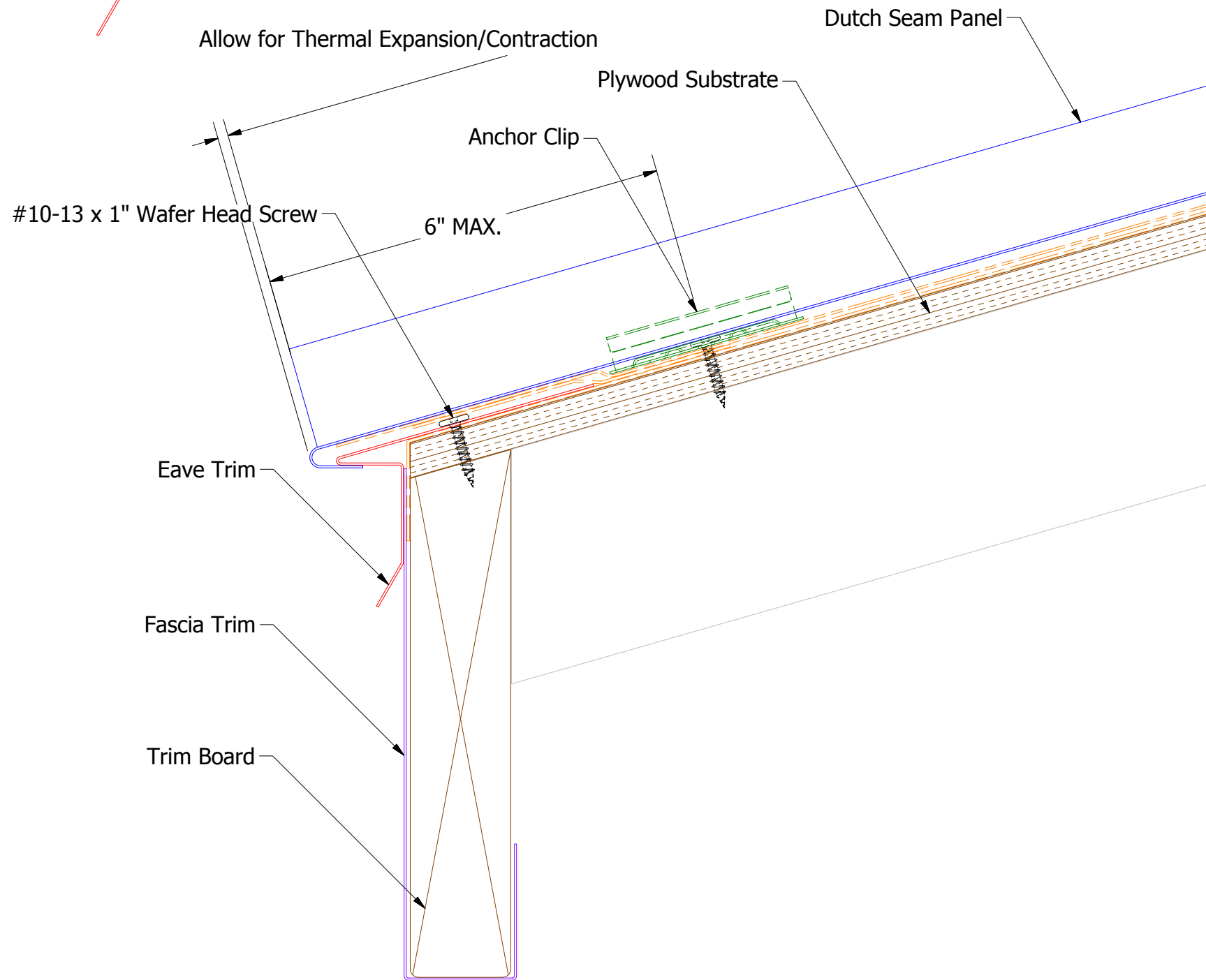
MDA115-Eave Trim without Return
