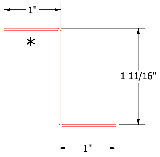
MDA910-Z Closure
