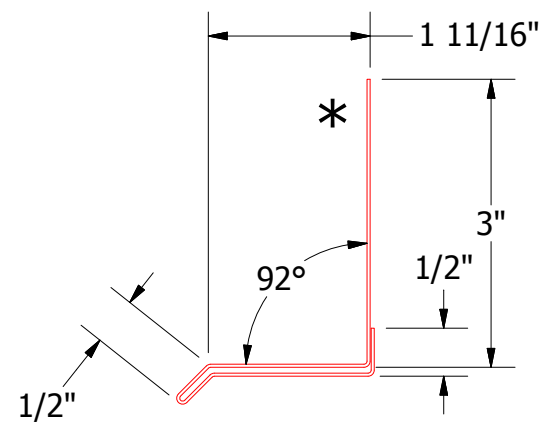
MDA661-Sill Trim with Return
