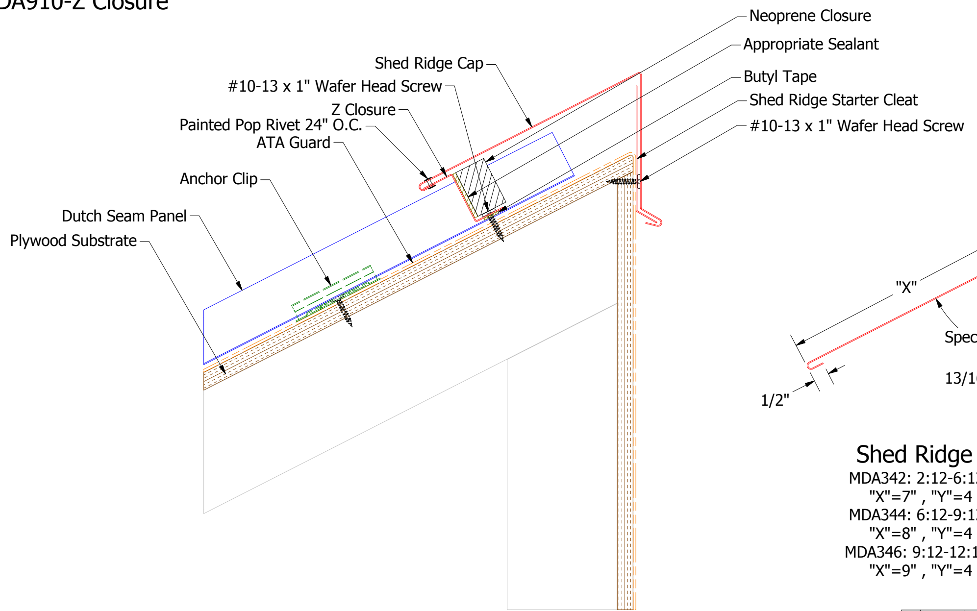
MDA910-Z Closure
