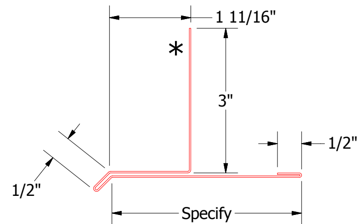
MDA662-T Sill Trim
