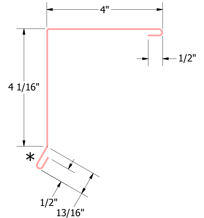
MDA210-Gable Trim Cap
