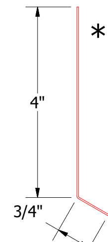
Shed Ridge Starter Cleat MDA341: For use with MDA342 Shed Ridge Cap MDA348: For use with MDA344 Shed Ridge Cap MDA349: For use with MDA346 Shed Ridge Cap
