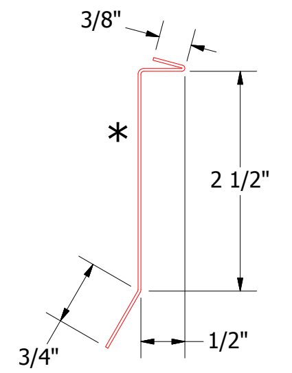
MDA980-Counterflashing
