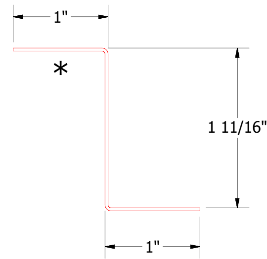
MDA910- Z Closure
