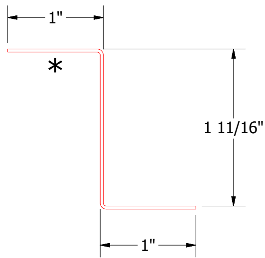
MDA910-Z Closure
