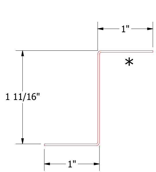
MDA910-Z Closure
