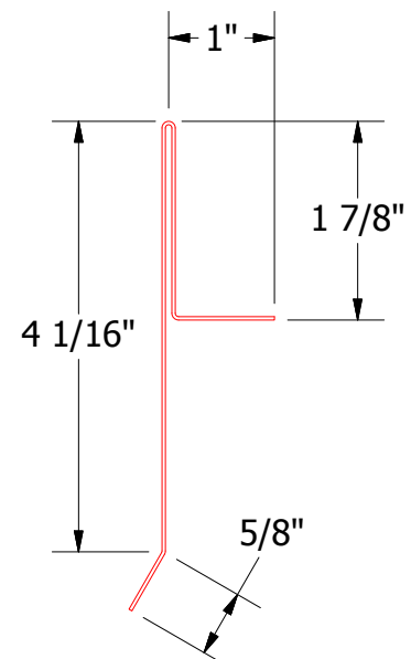
MDA211-Gable Trim Starter Cleat
