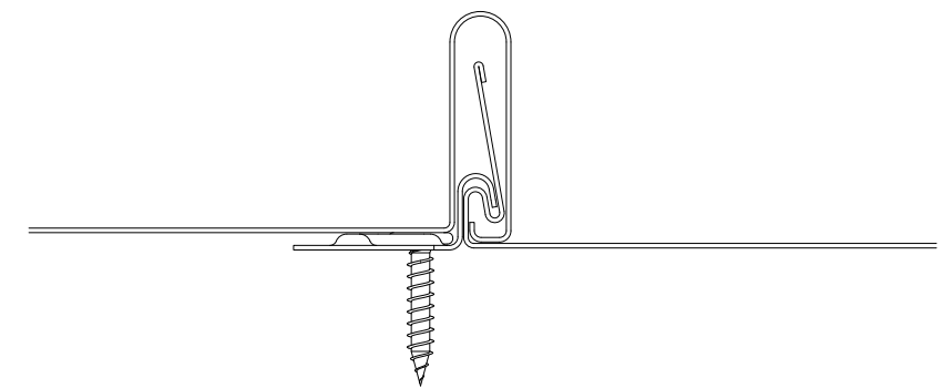
Positive Panel Interlock
