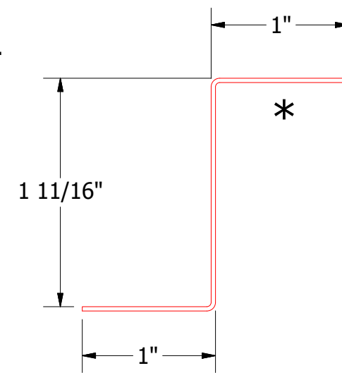
MDA910-Z Closure
