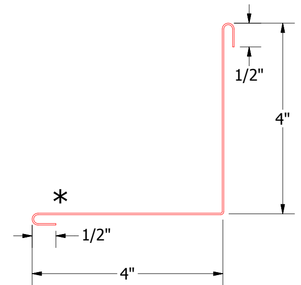
MDA600-Inside Corner Cap
