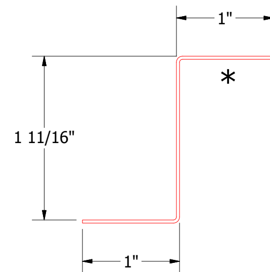
MDA910-Z Closure
