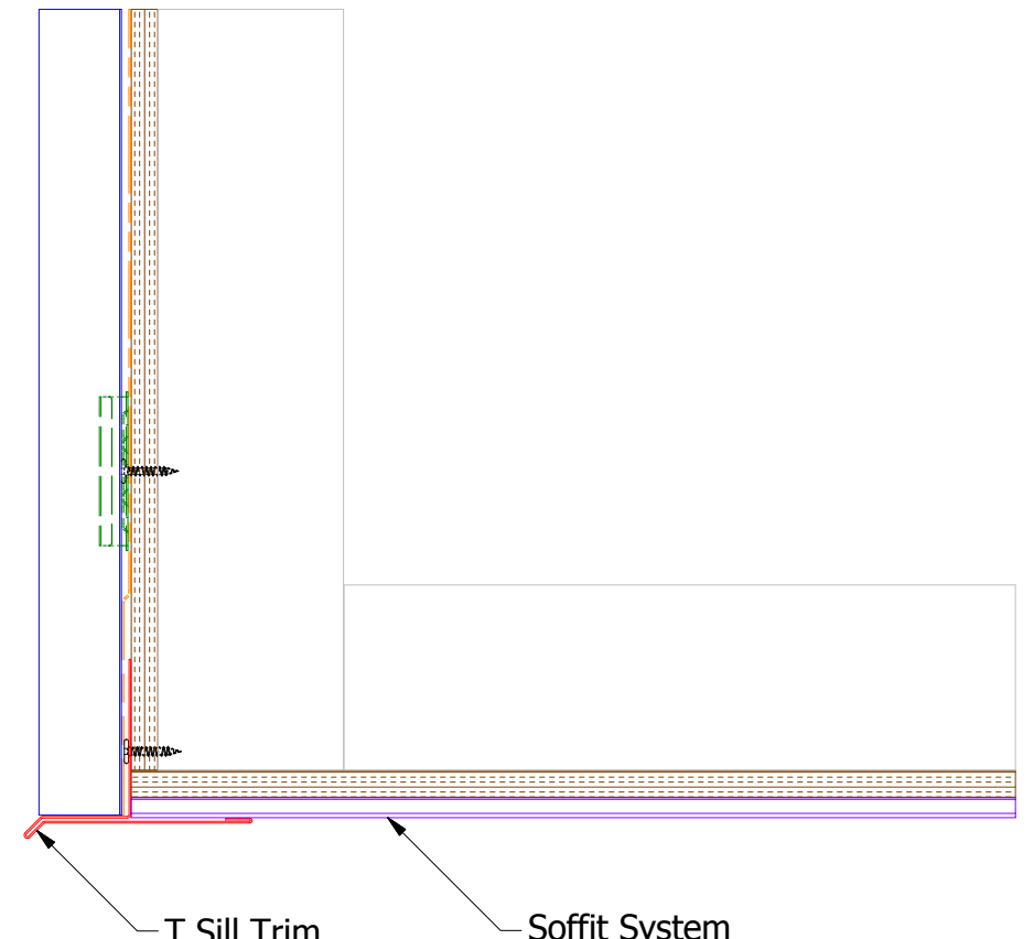
Sill Trim with Return
