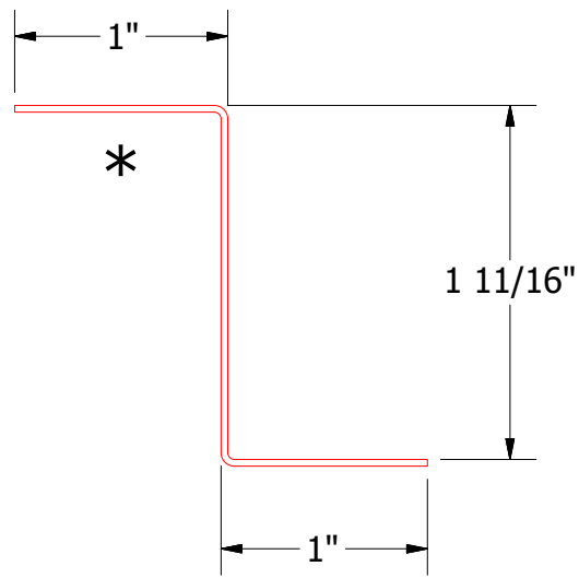
MDA910-Z Closure
