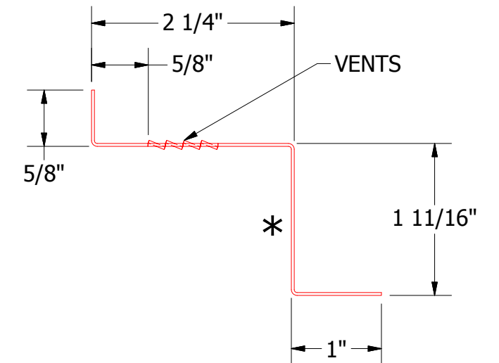
MDA911-Vented Z Closure
