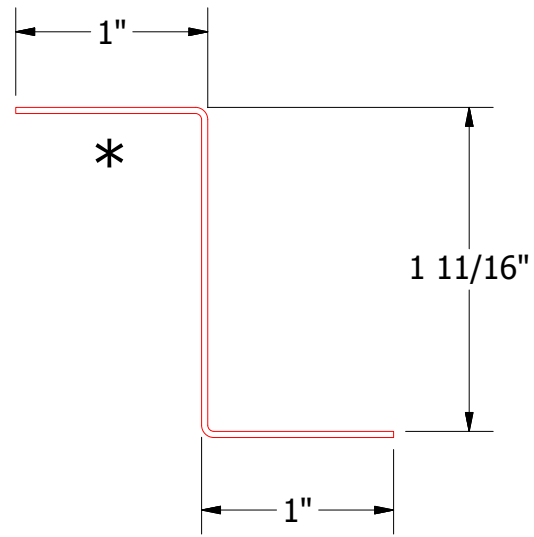
MDA910-Z Closure
