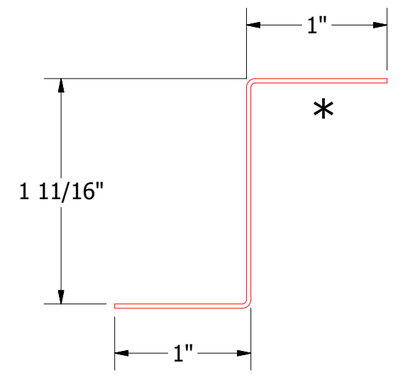
MDA910-Z Closure
