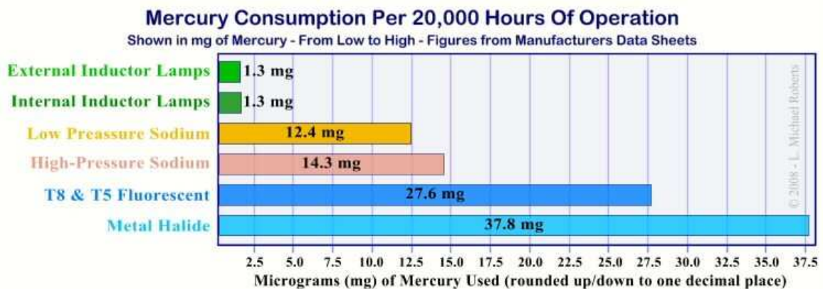
Fig. 7 - Mercury Consumption Per 20,000 Hours of Operation for Various Lamp types Click image to see full size version
