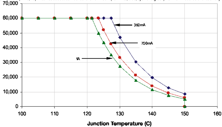
Figure 9. Expected (B10, L70) lifetimes for InGaN LUXEON Rebel.
