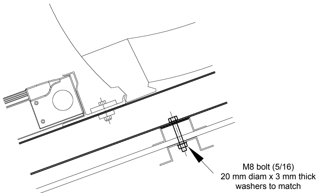
Diagram 15 – On Roof Mounting Bolt into Steel Batten
