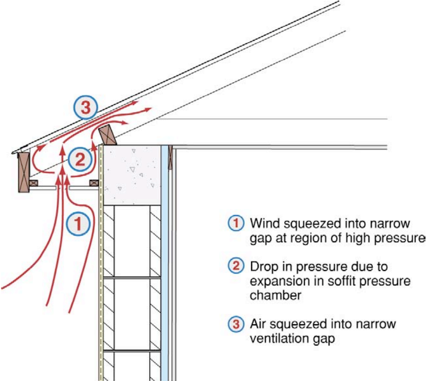
Figure 16: Pressure Relieved – Baffled Soffit Assembly
