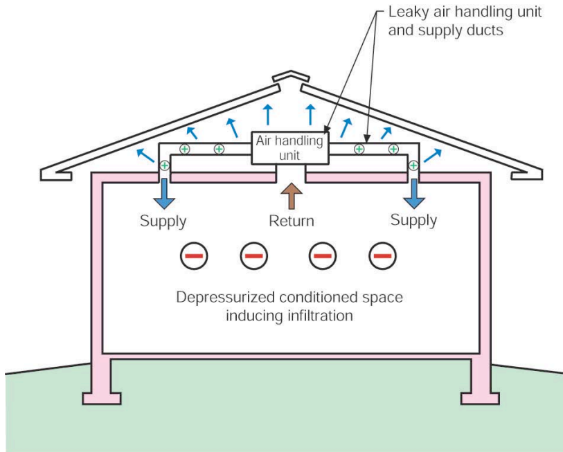
Figure 18: Negative Pressure Induced Via Duct Leakage
