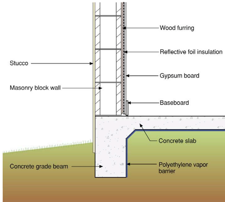
Figure 2: Mass Assembly
