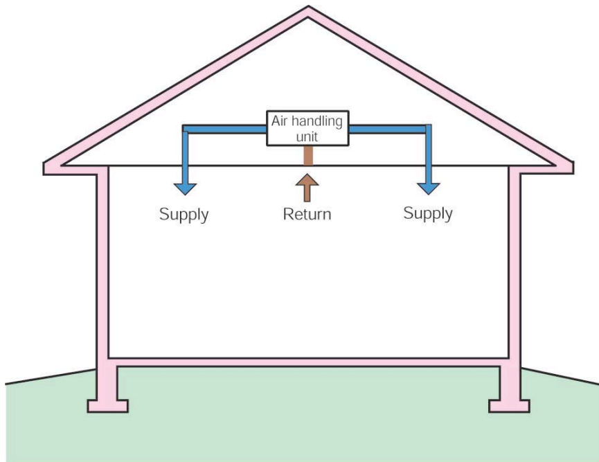
Figure 19: Conditioned Unvented Attic Assembly
