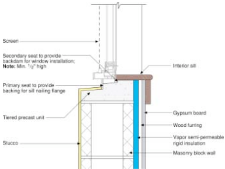
Figure 14: Recommended Practice That Directs Window Leakage Outward
