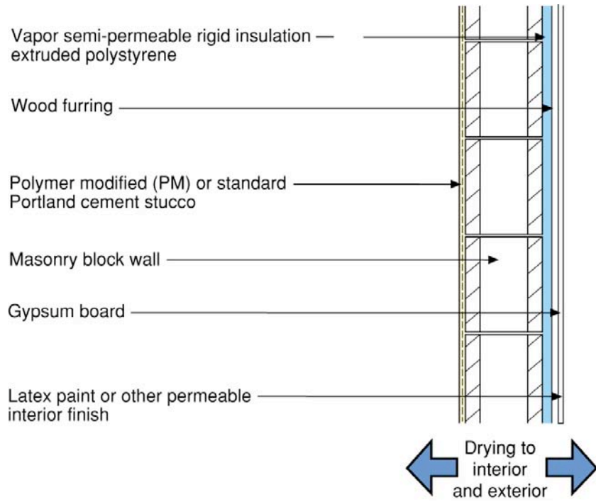
Figure 22: Vapor Semi Permeable Non Water Sensitive Rigid Insulation
