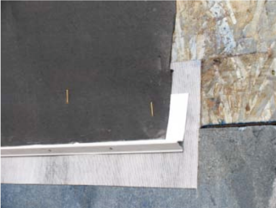
Photograph 20: Primary Drainage Plane Lapped Over Control Joint Flashing
