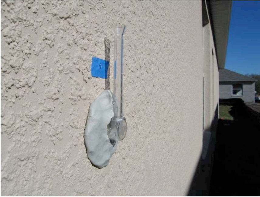
Photograph 43: Rilem Tube Hydrostatic Head Test
