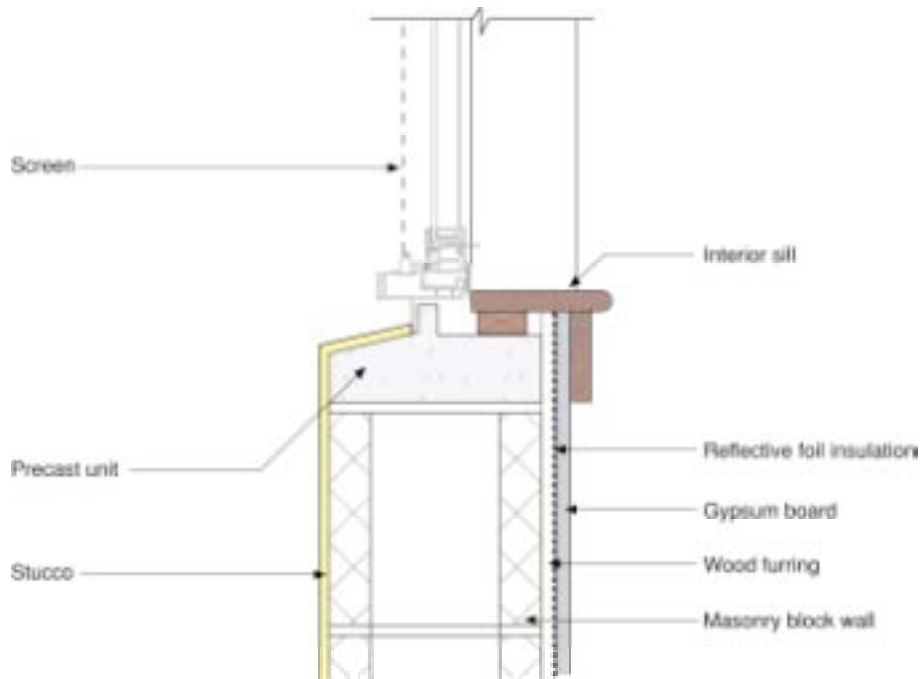
Figure 13: Current Practice That Directs Window Leakage Inward
