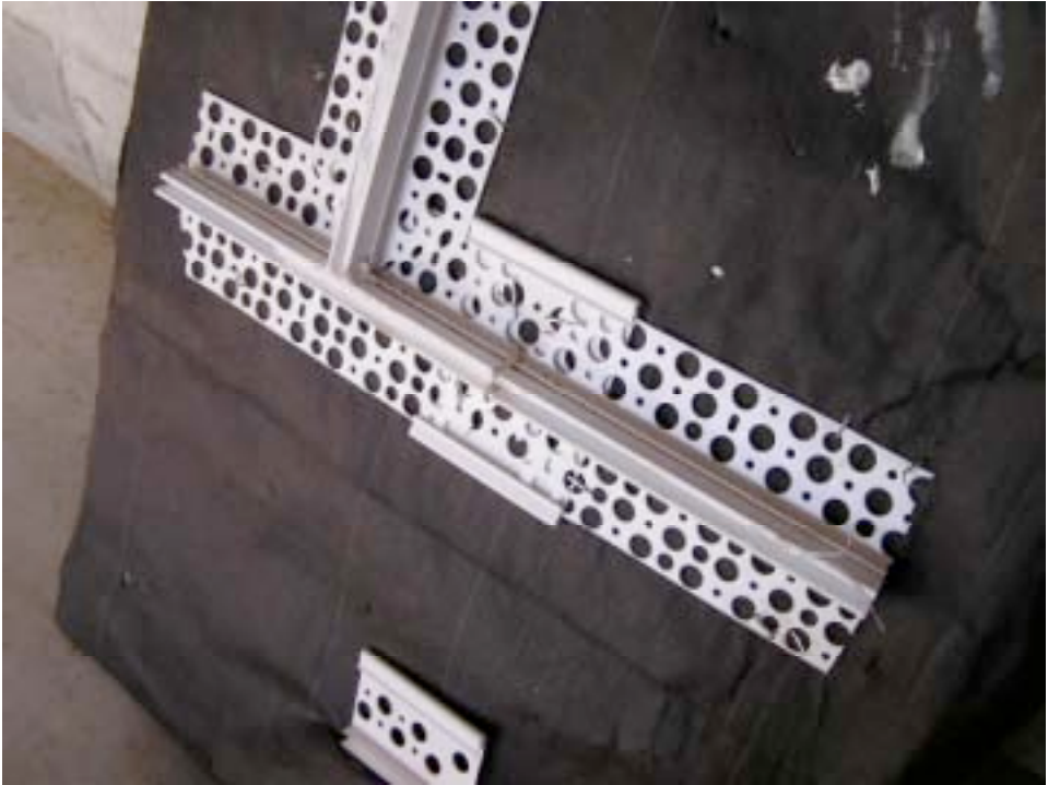
Photograph 15: Control Joint Accessories Installed Over Top of Drainage Plane
