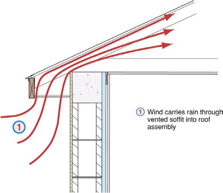
Figure 15: Wind Driven Rain Entry In Vented Soffit Assembly
