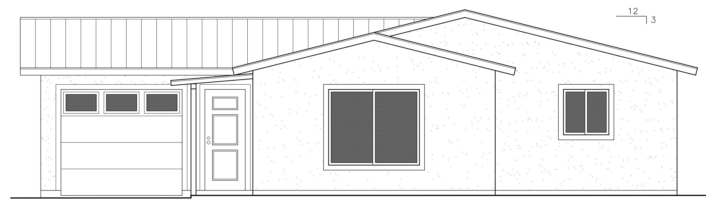
Front Elevation 1/4" = 1'-0"
