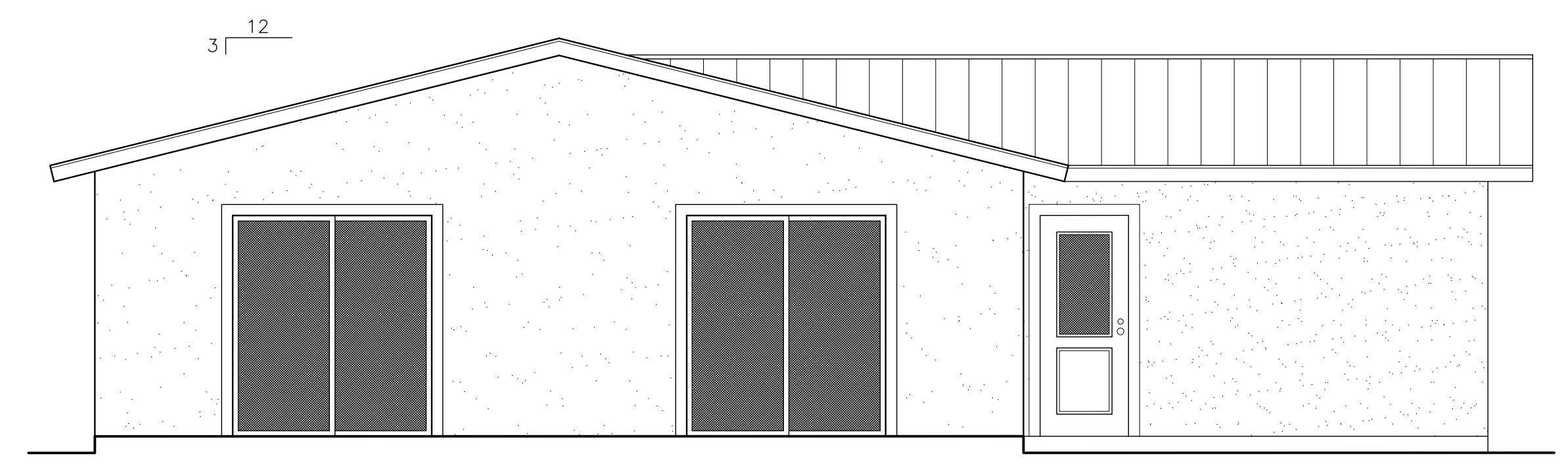
Back Elevation 1/4" = 1'-0"
