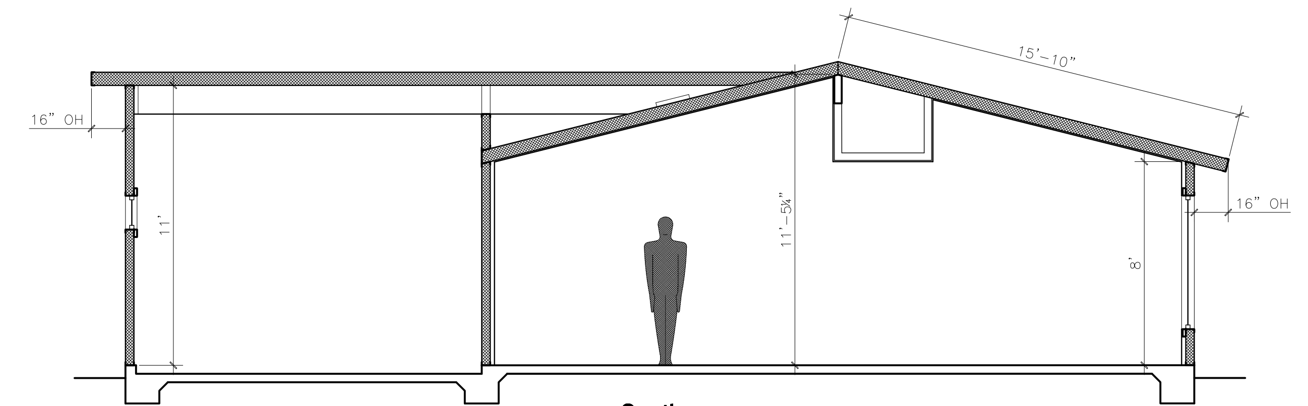
Section 1/4" = 1'-0"
