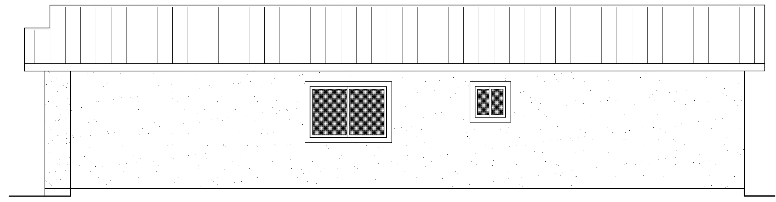
Right Elevation 1/4" = 1'-0"
