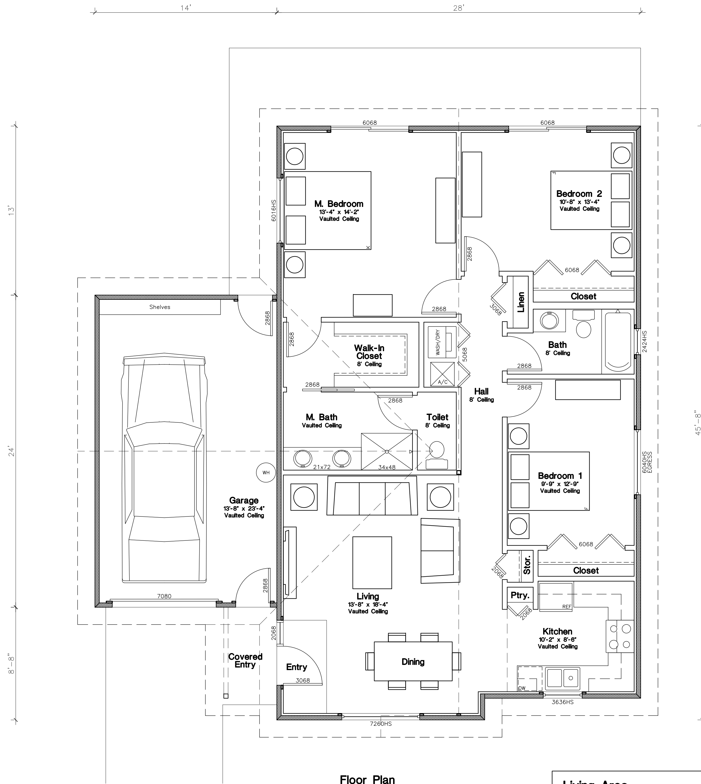
Floor Plan 1/4" = 1'-0"
